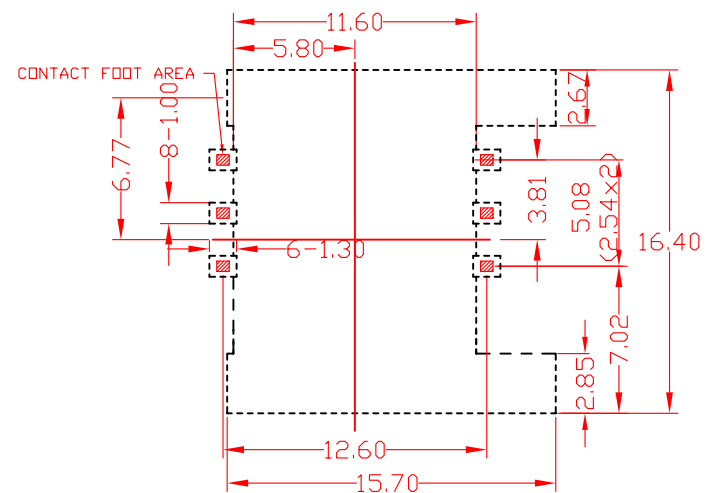
The recommended pcb layout (Tolerance=±0.1mm)
