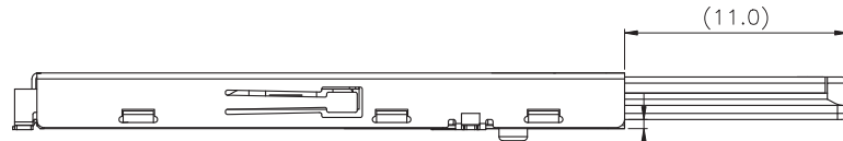
SD CARD -Un Lock
