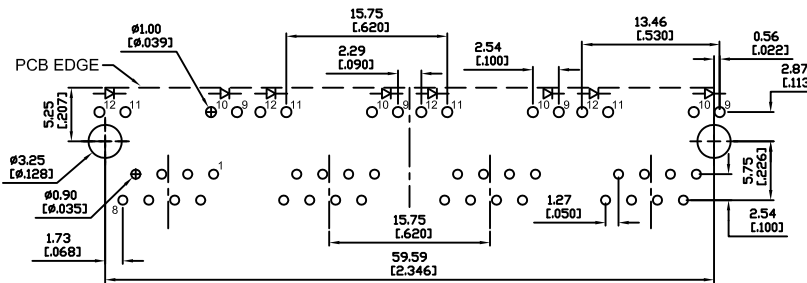
SUGGESTED PCB LAYOUT TOP VIEW
