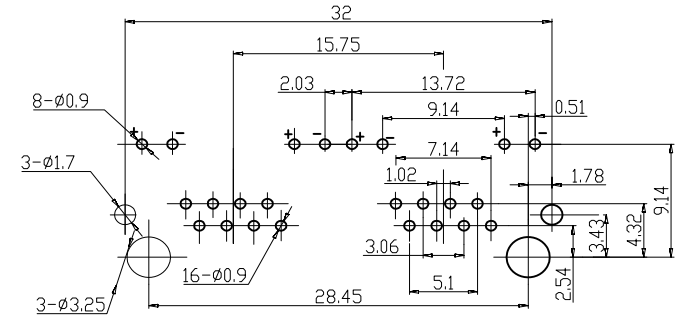
PCB LAYOUT
